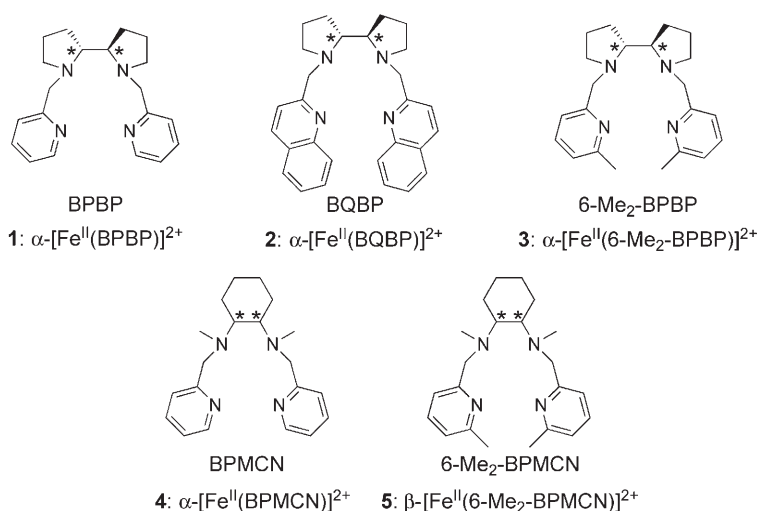
Figure 1. Optically active ligands (chiral centers indicated by *) and their corresponding iron complexes (in which the ligand coordinates in either a cis - \alpha or cis - \beta topology) capable of promoting asymmetric olefin cis -dihydroxylation.
